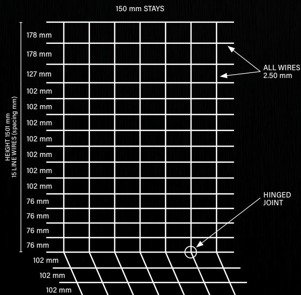
FERAL BLOC - 15 / 150 / 15 WITH FOOTER Graduated Line Wire Spacings Purpose: Wild Dogs, Pigs, Kangaroos
